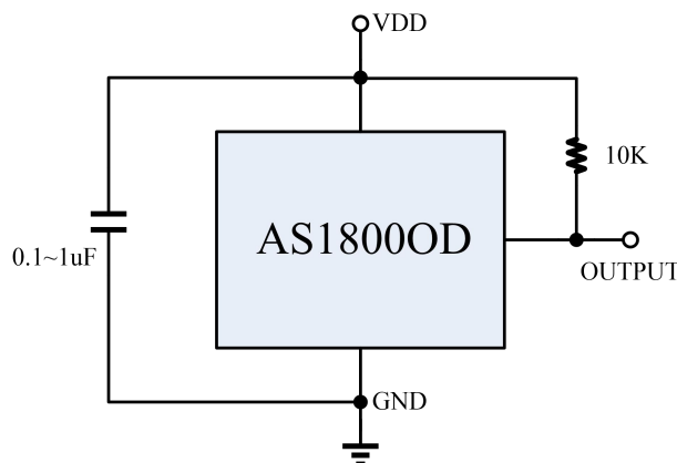
Figure 1, Typical Application Circuit of AS1800OD
