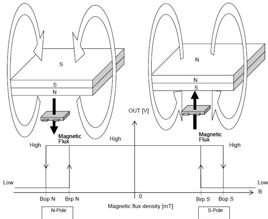
Fig 4, Magnetic Operation Characteristic of AS1800OD
