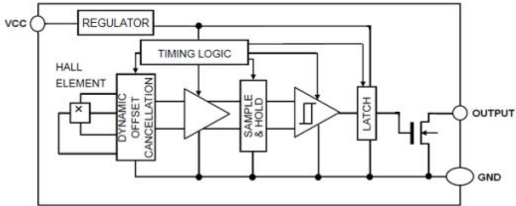
Figure2, Block Diagram of AS1800OD
